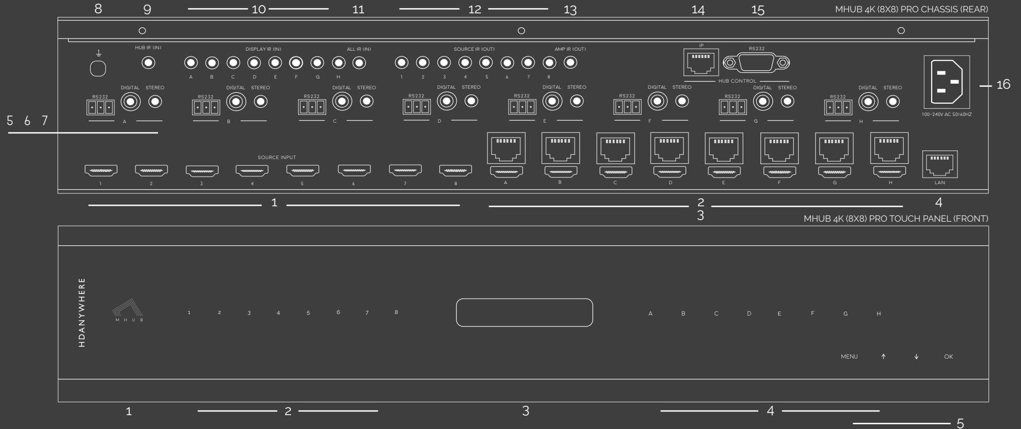
MHUB 4K (8X8) CHASSIS (REAR)
